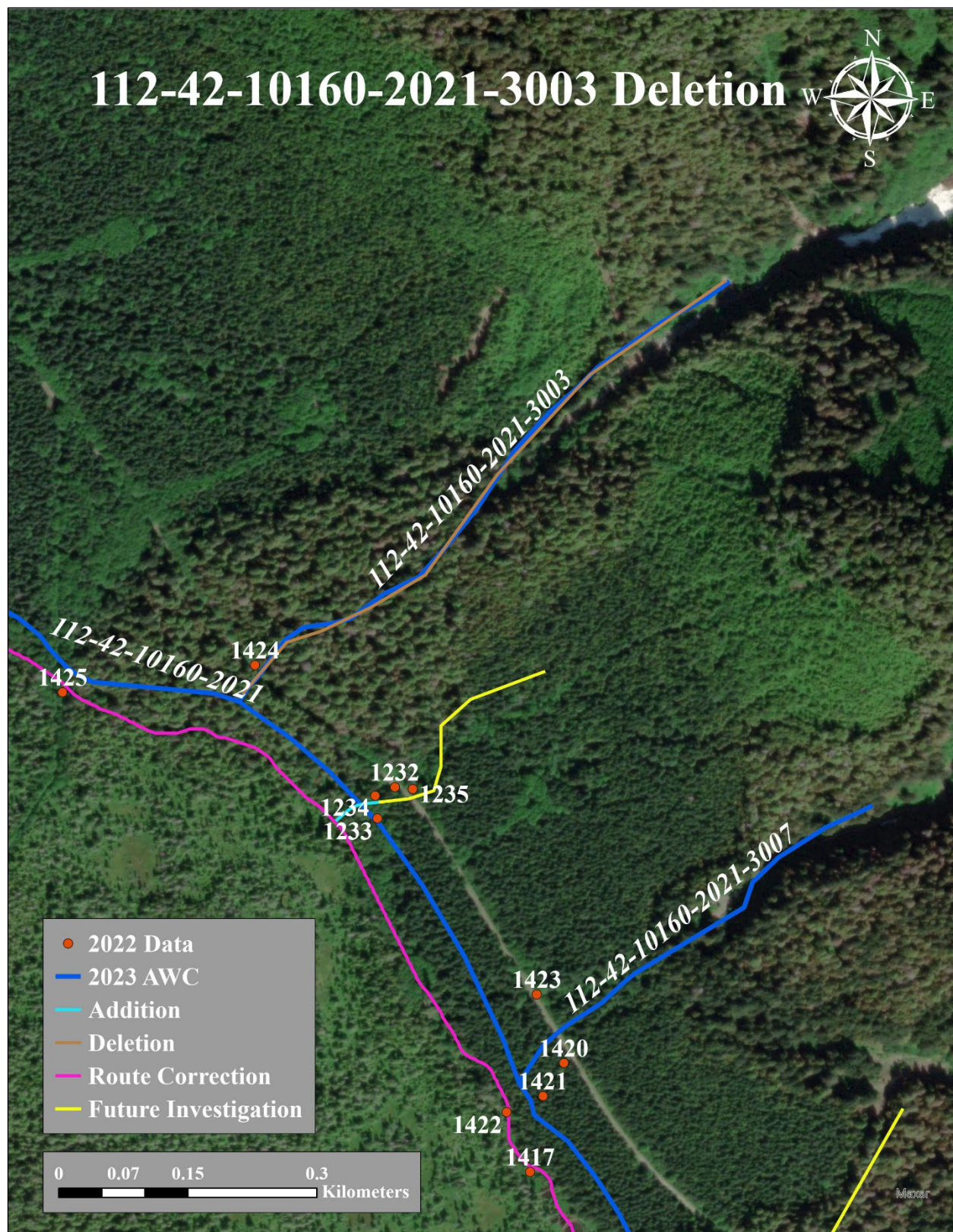
Figure 1.–112-42-10160-2021-3003 deletion map.
